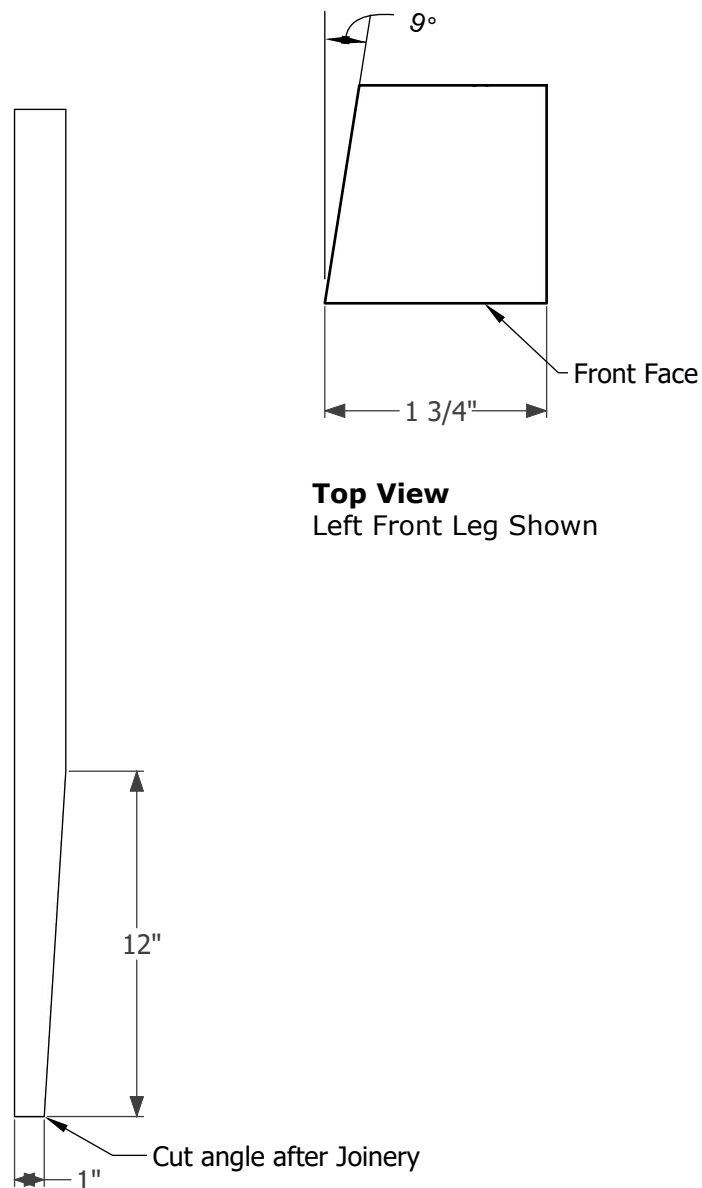
Front Face Left Front Leg Shown
