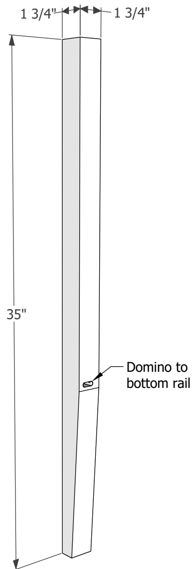
Perspective Left Front Leg Shown
